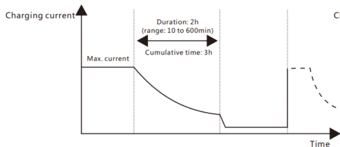
Fig. 1-5 SLD Battery charging stages diagram
