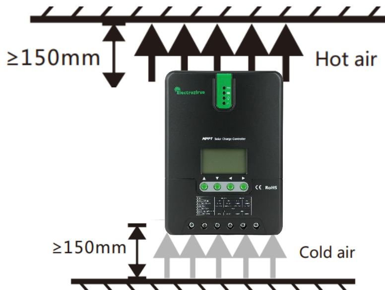
Figure 2.1 Installation and Heat Dissipation
